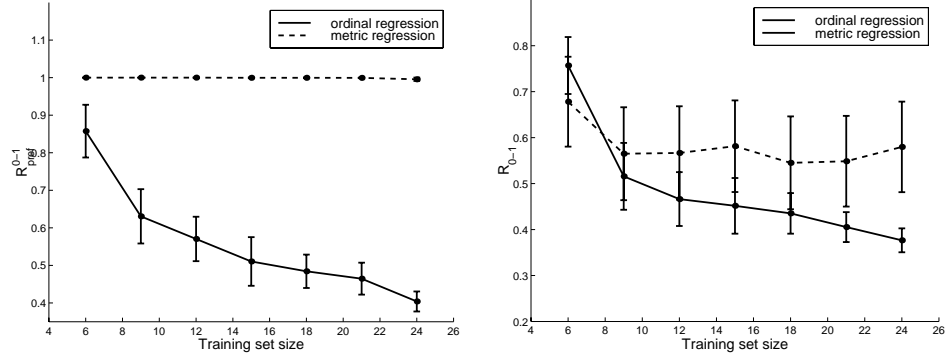
Figure 2.5 Learning curves for SVR (dashed lines) and the algorithm for ordinal regression (solid line) for the OHSUMED dataset query 1 if we measure (a) R_{\text{pref}} and (b) R_{0-1} . Error bars indicate the 95% confidence intervals.
