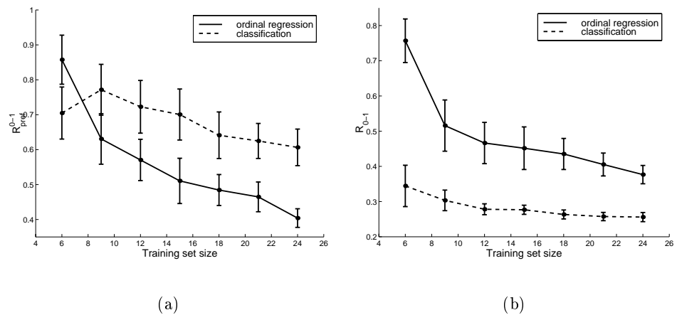
Figure 2.4 Learning curves for multi-class SVM (dashed lines) and the algorithm for ordinal regression (solid line) for the OHSUMED dataset query 1 if we measure (a) R_{pref} and (b) R_{class} . Error bars indicate the 95% confidence intervals.
